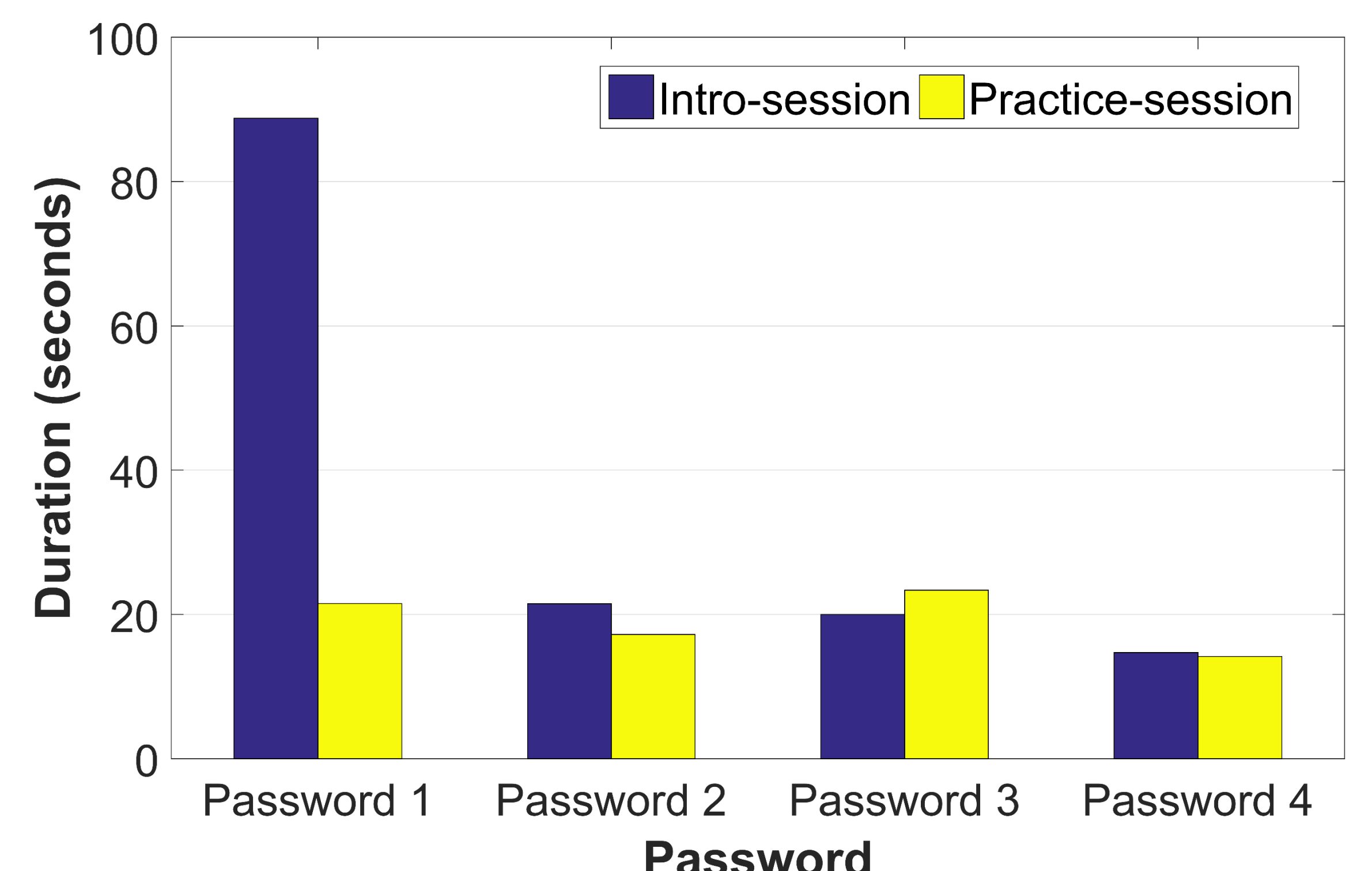
Average time spending on each password
